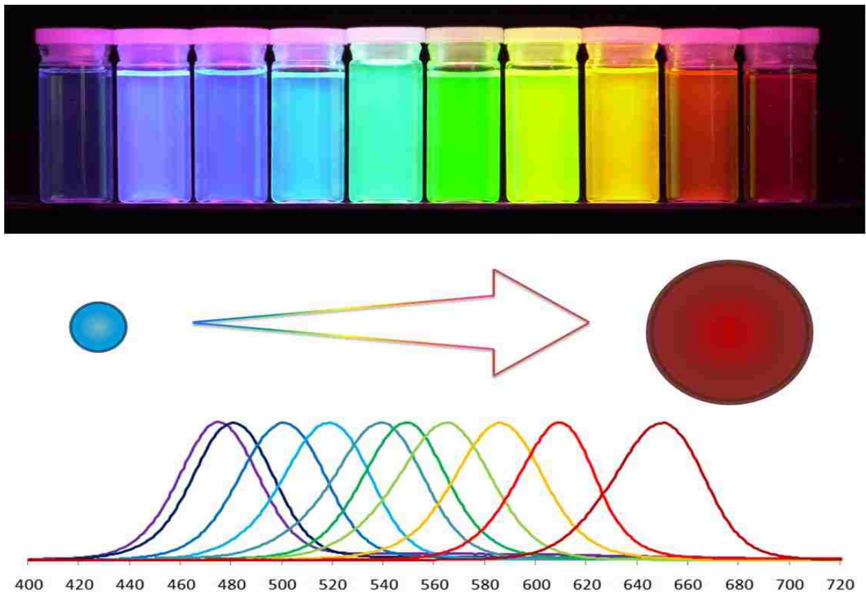
Figure 1.3 Unique photo-physical properties of QDot probes. Direct correlation between the nanoparticle size and the wavelength of emitted photon, originating from the quantum confinement of charge carriers, offers precise control over QDot color and yields narrow symmetrical light emission profiles (bottom). Wide absorption profile, in turn, allows simultaneous excitation of multicolor QDots with a single high-energy light source (top).
